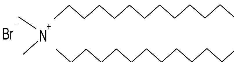
Figure 1: Structure of N, N-didodecyl-N, N-dimethylammonium bromide coating
